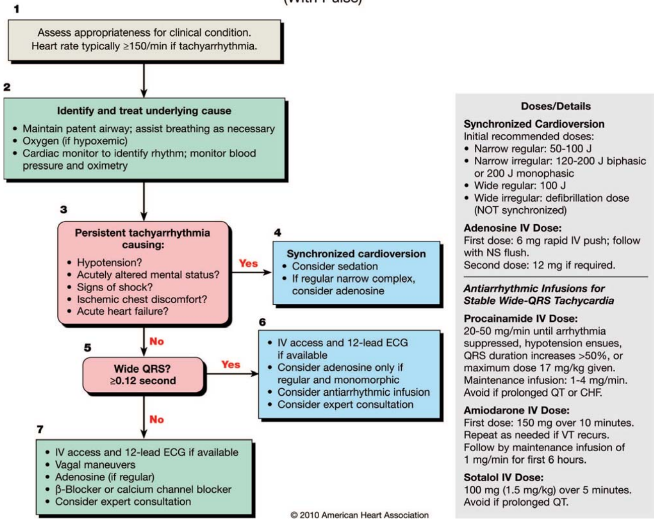
Figure 4. Tachycardia Algorithm.
